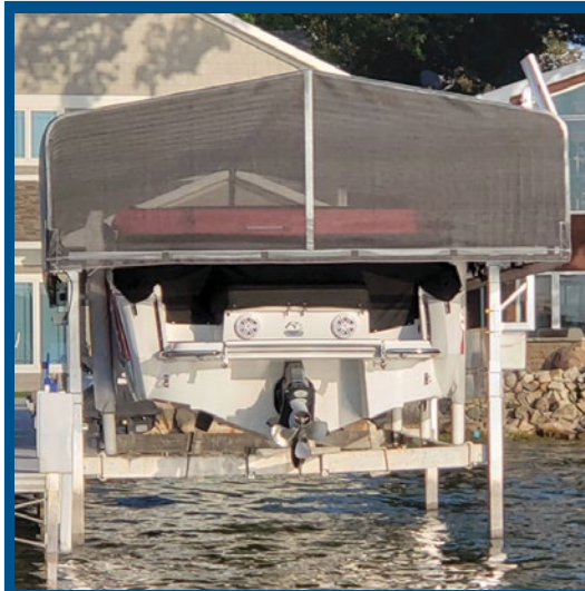
V-Boat Lifting Bunks
